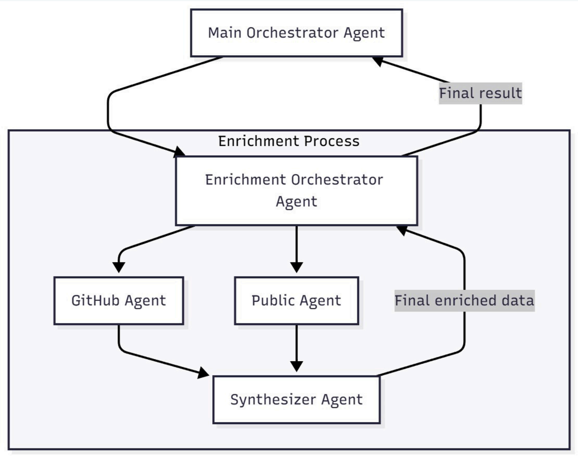
Enrich resume flow chart
