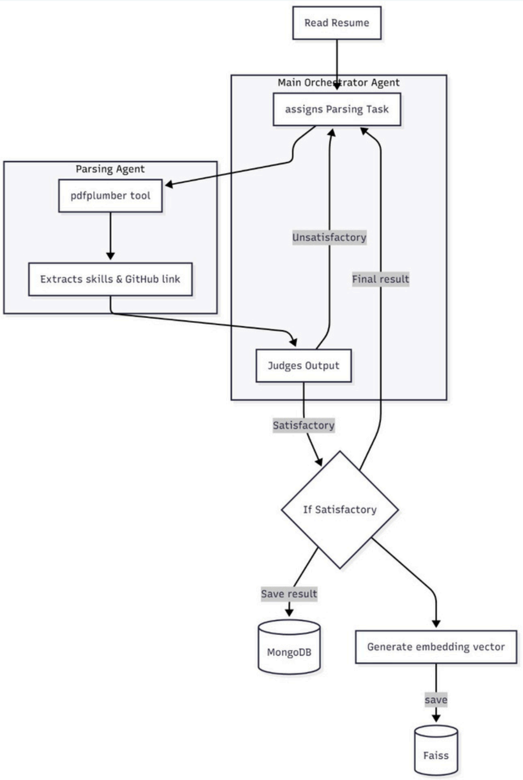
Parse resume flow chart
