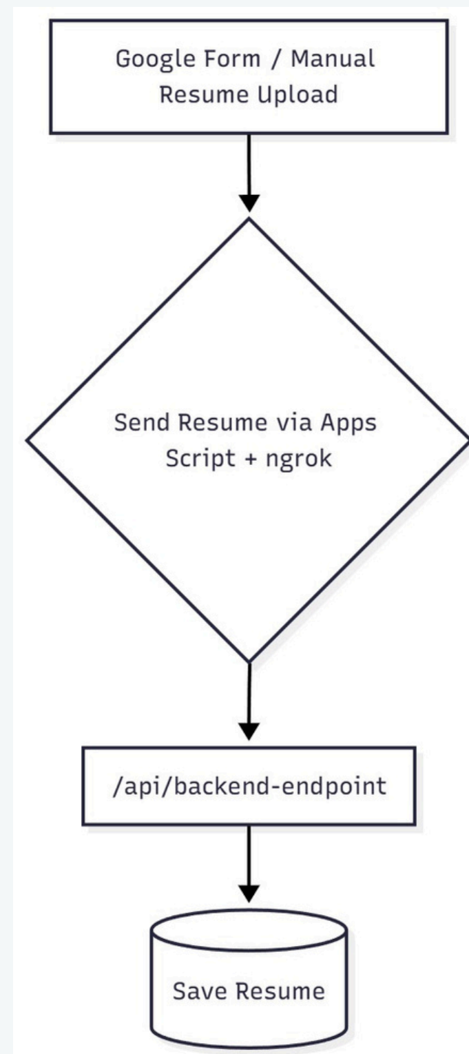
Upload resume flow chart
