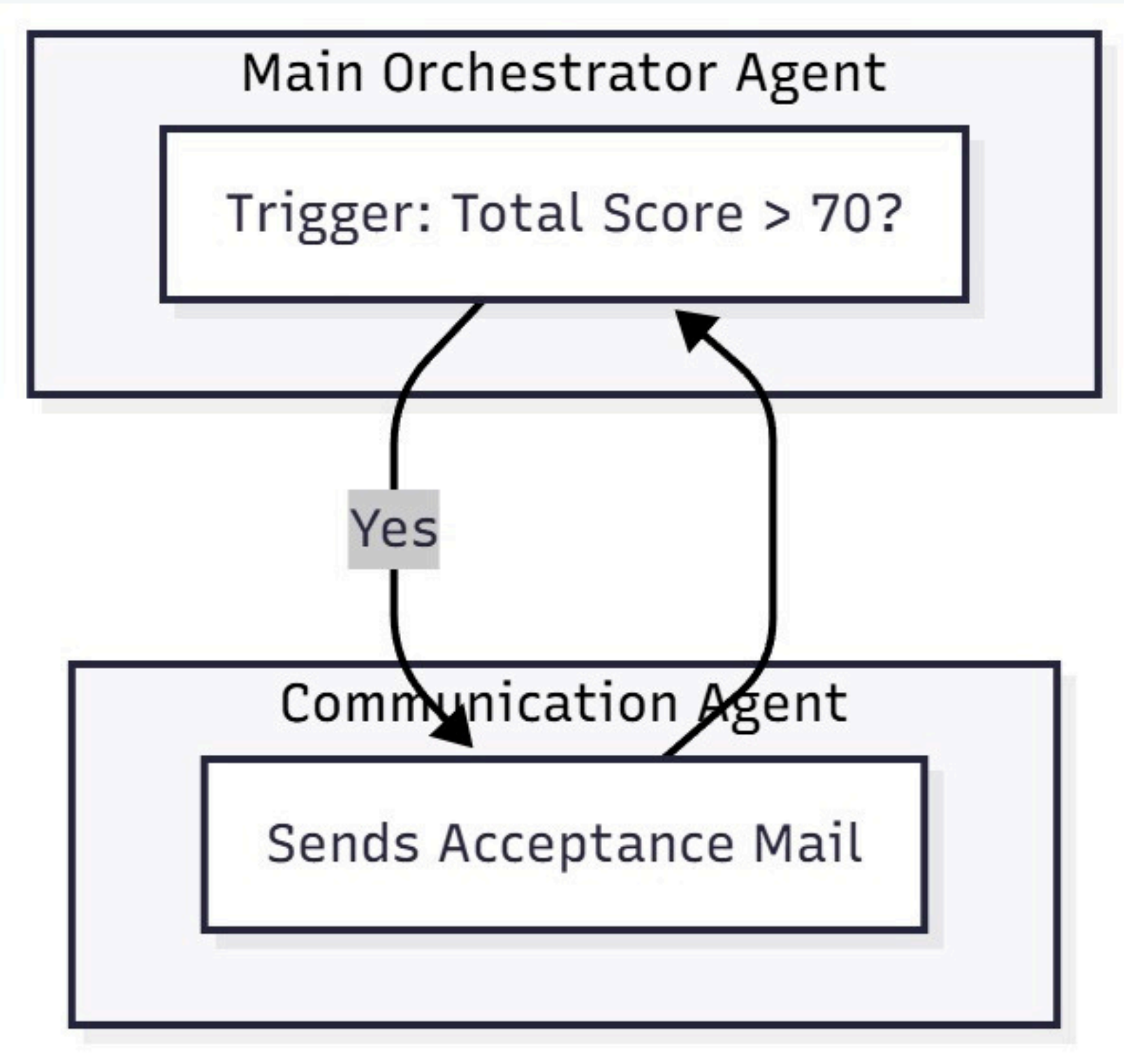
Send final acceptance mail flowchart
